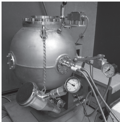
Siwek 20L Sphere
